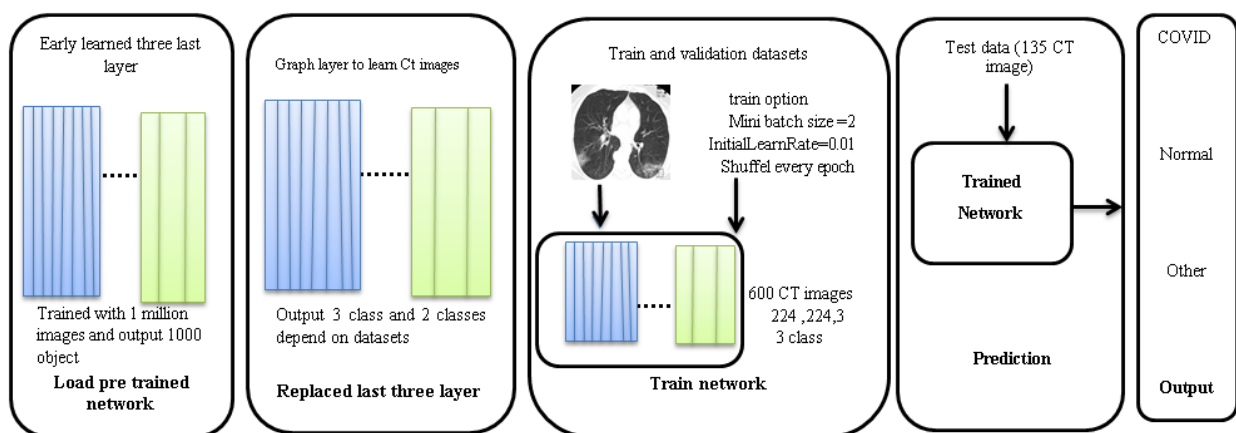
Figure 3: Modified ResNet 50 network for detection
